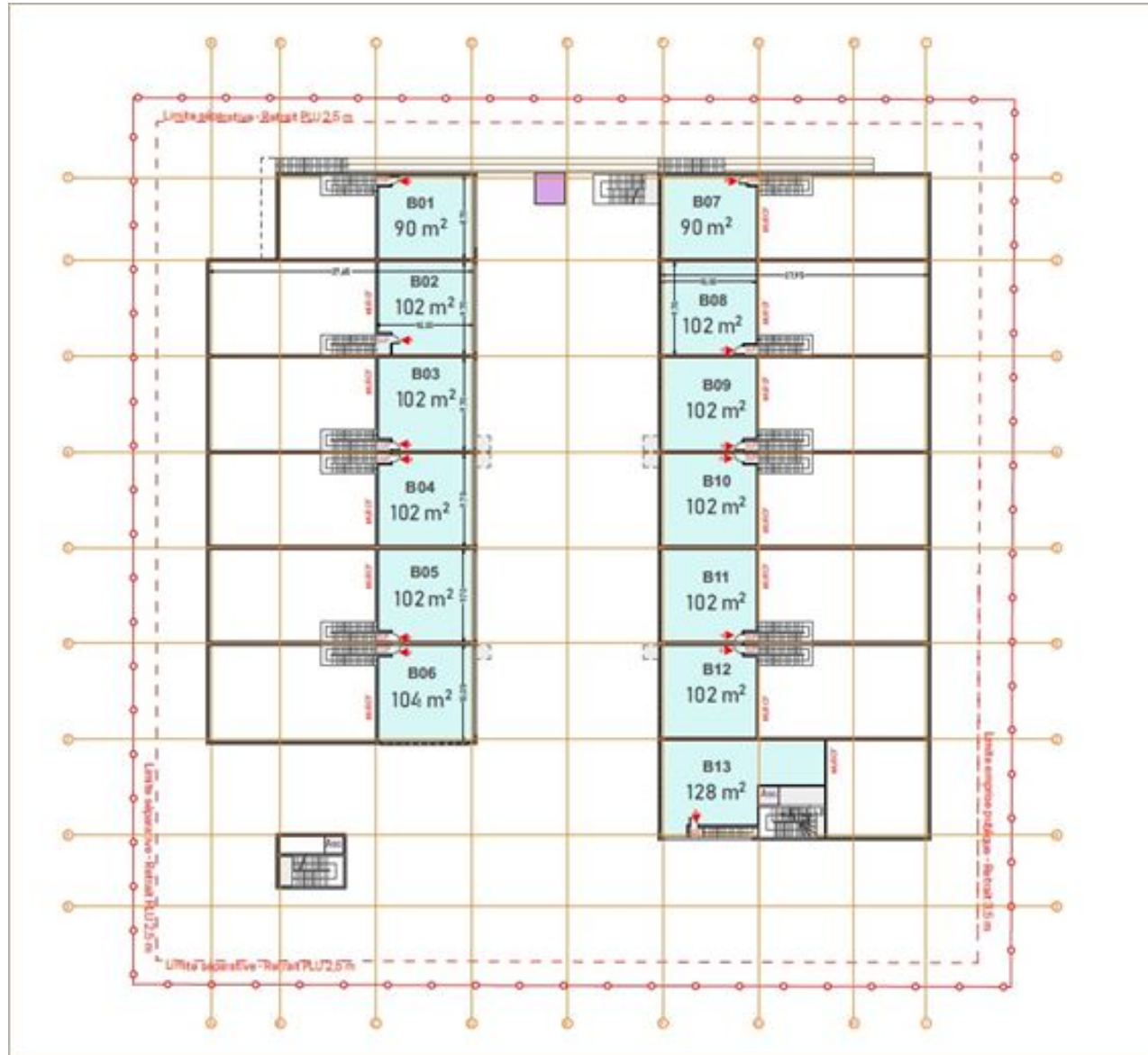
Plan r+3
