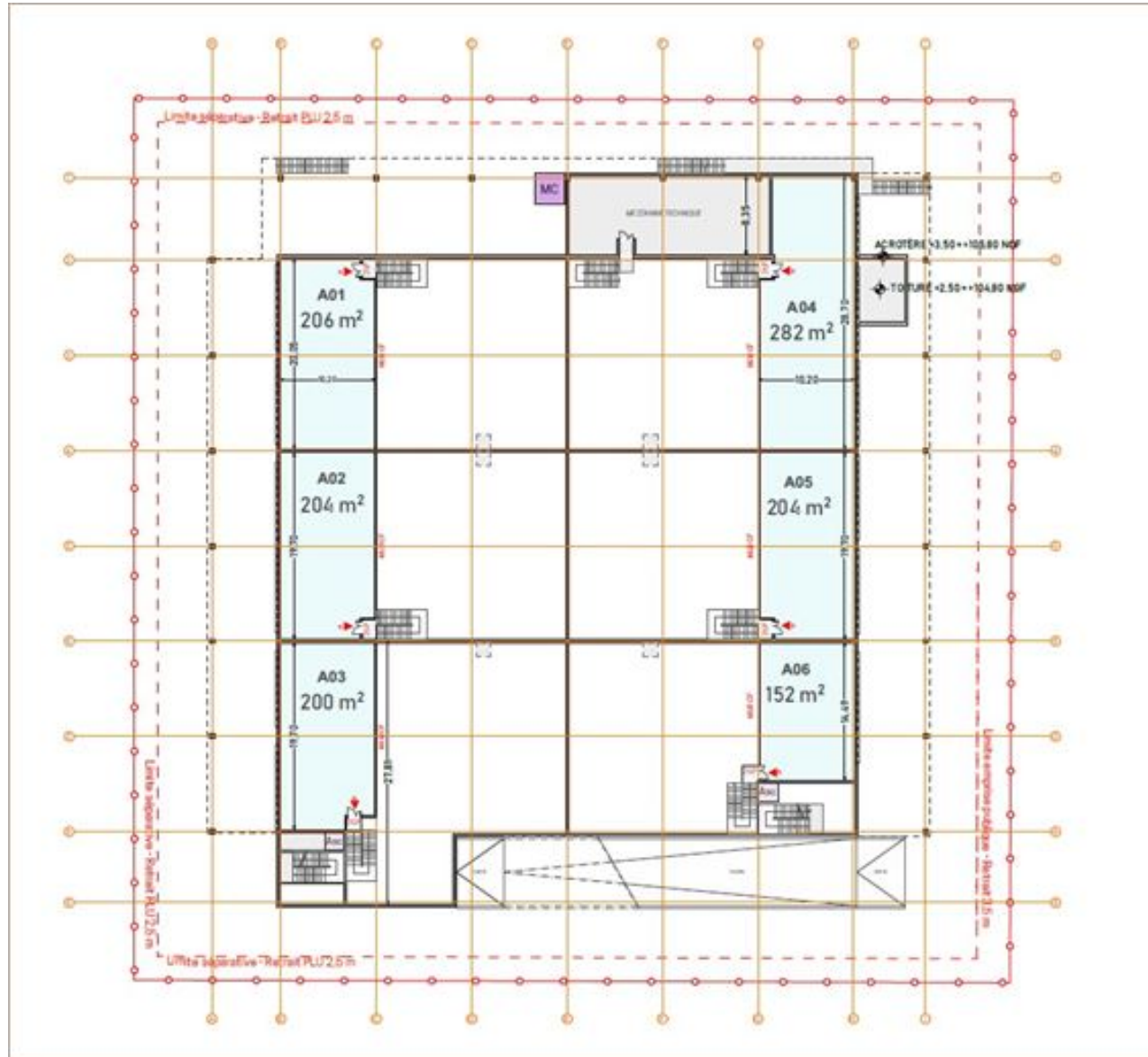
Plan r+1
