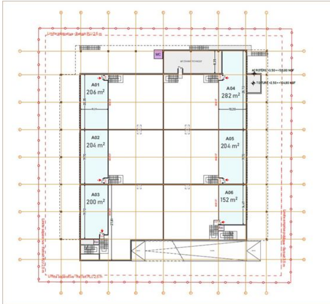
Plan r+1
